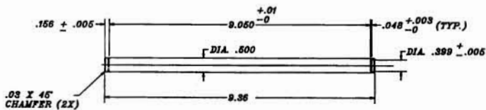
⑥ MAT'L. 1/2" DIA. C.R. STEEL 2 REQ'D. BLACK OXIDE/OIL
