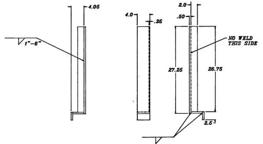
DETAIL B WELDMENT
