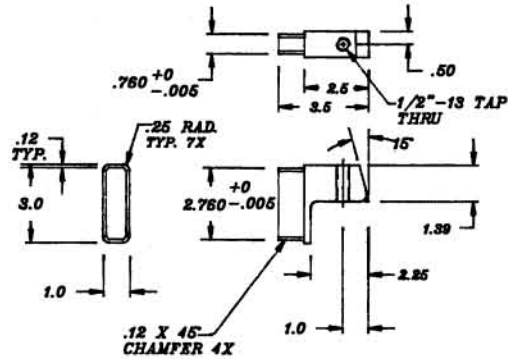
⑧ MAT'L 1 X 3 C.R. STEEL 2 REQ'D.
