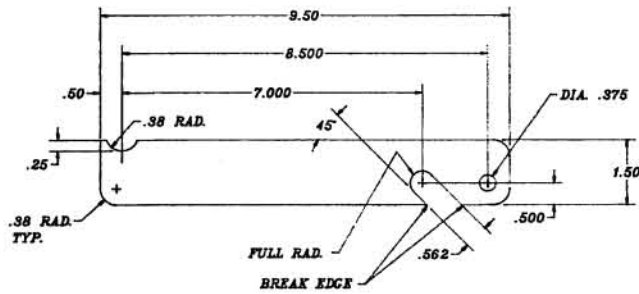
① MAT'L. 1/4" THK X 1.5" C.R. BAR 2 REQ'D.
