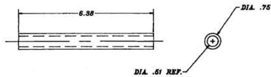
② MAT'L. TUBE, 3/4" OD. X .120 WALL DOM STEEL 1 REQ'D.
