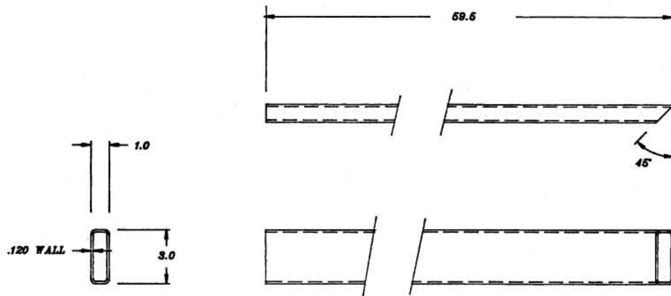
⑥ MAT'L TUBE 1" X 3.0" X .120 WALL E.W. STEEL 3.07# / FT. 2 REQ'D.
