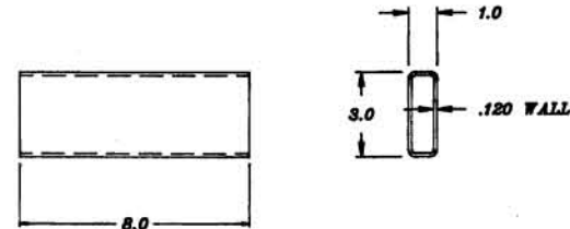
⑩ MAT'L TUBE 1" X 3" X .120 WALL E.W. STEEL 3.07# / FT. 2 REQ'D.
