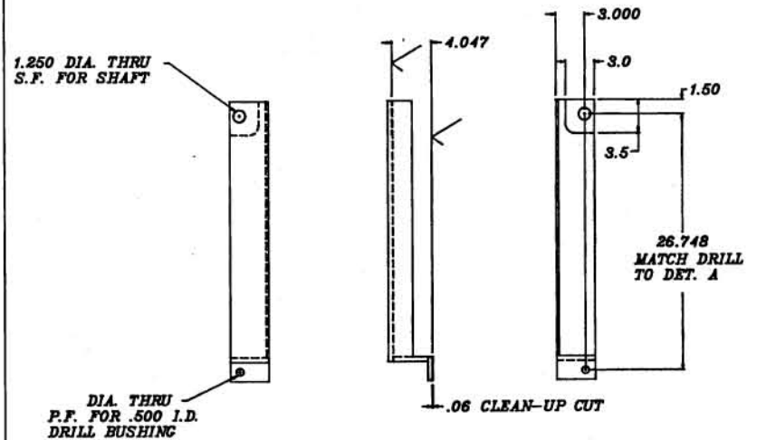
DETAIL B MACHINING
