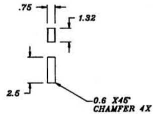
⑪ MAT'L .75 THK H.R. STEEL 1 REQ'D.
