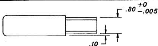
9 MAT'L. TUBE 1 X 3 X .094 WALL EW STEEL 2 REQ'D.
