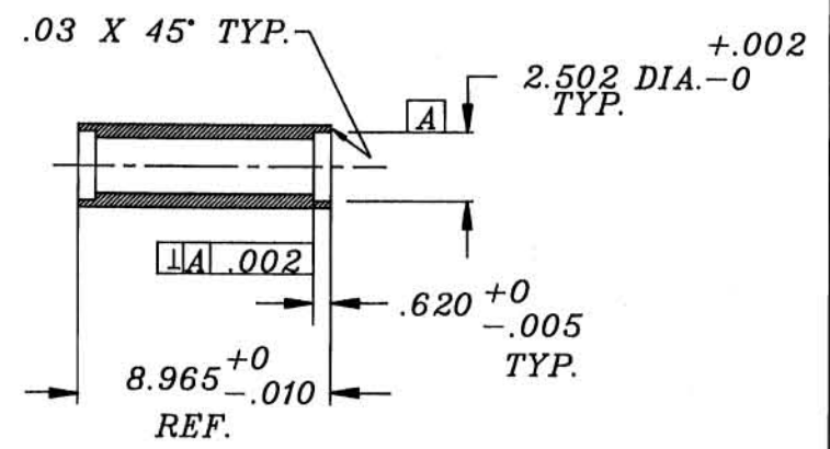
DETAIL OF BEARING HOUSING
