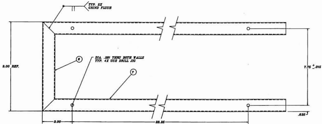
ALIGN HOLES WITH 1/2" ROD PRIOR TO WELDING 2X
