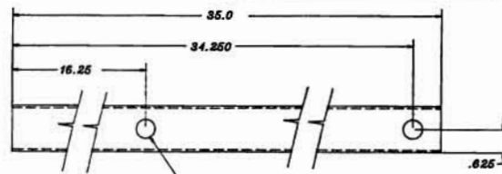
DIA. .515 THRU BOTH WALLS TYP. 2X MATCH DRILL 2 PIECES
