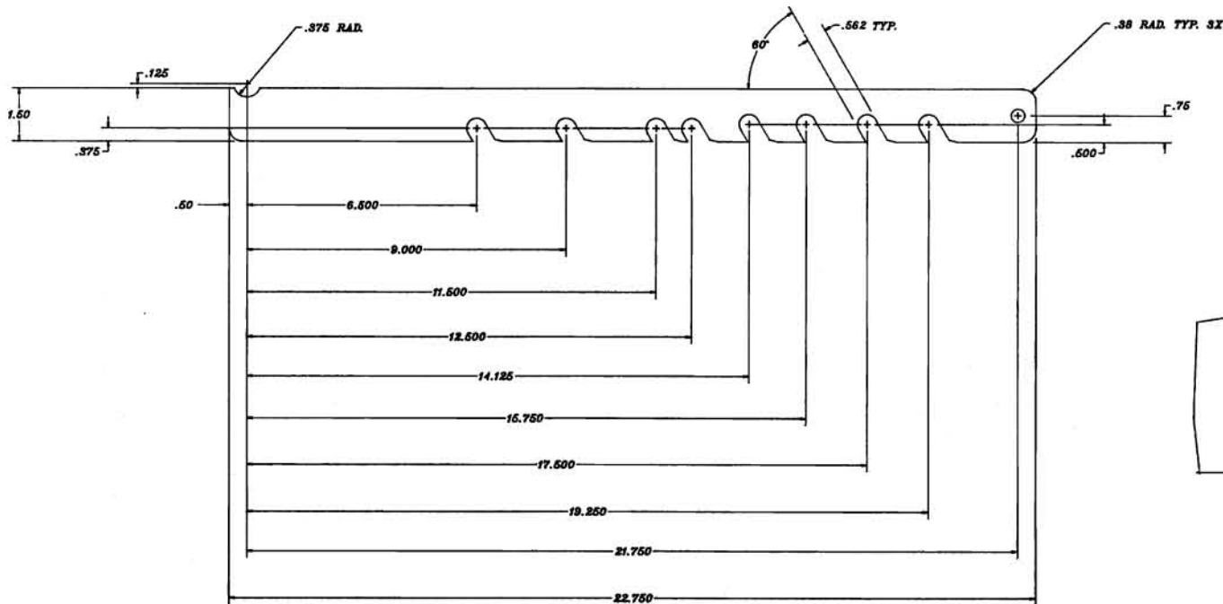
NOTCH DETAIL TYP. 3X
