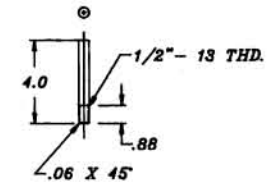
⑩ MAT'L .50 DIA. C.R.S. 1 REQ'D.
