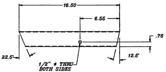
② MAT'L TUBE, 2.50" SQ. X .094 WALL E.W. STEEL 1 REQ'D.
