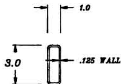
⑦ MAT'L TUBE 1" X 3.0" X .120 WALL E.W. STEEL 3.07 # / FT. 1 REQ'D.
