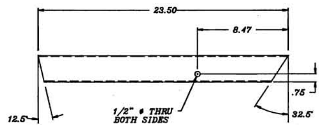
③ MAT'L TUBE, 2.50" SQ. X .094 WALL E.W. STEEL 1 REQ'D.
