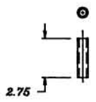
⑧ MAT'L TUBE, .688 OD. X .51 ID. SEAMLESS STEEL 4 REQ'D.
