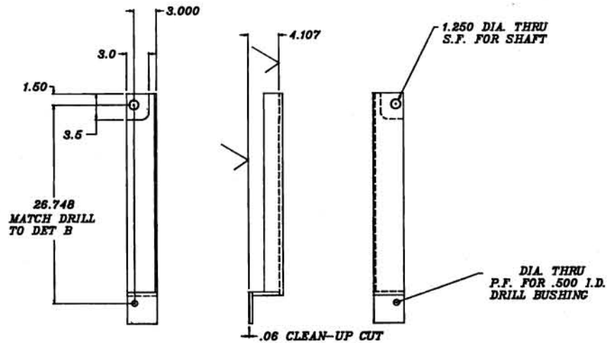
DETAIL A MACHINING
