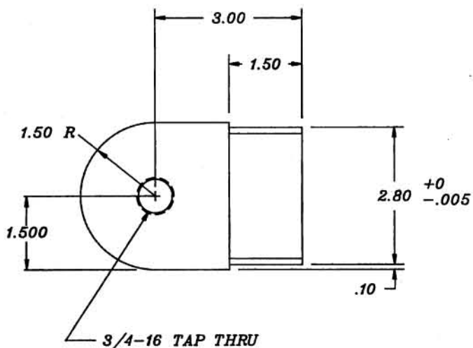
10 MAT'L. 1 X 3 BAR C.R. STEEL 2 REQ'D.
