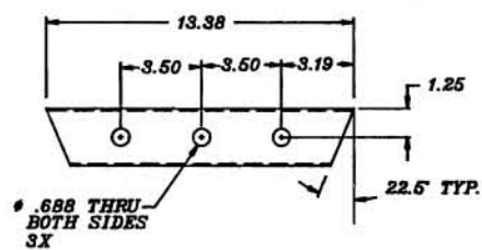
④ MAT'L TUBE, 2.50" SQ. X .094 WALL E.W. STEEL 1 REQ'D.
