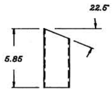
① MAT'L TUBE, 2.50" SQ. X .094 WALL E.W. STEEL 1 REQ'D.
