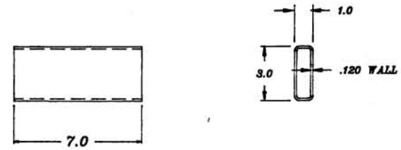
⑨ MAT'L TUBE 1" X 3" X .120 WALL E.W. STEEL 3.07# / FT. 2 REQ'D.
