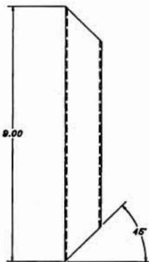
⑤ MAT'L. TUBE 1.25 SQ. X .085 WALL KW STEEL 1 REQ'D.
